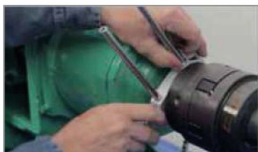
1. Mount the V-brackets
